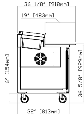
FPT- SECTION
