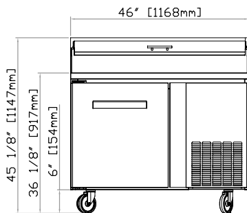
FPT-46 FRONT
