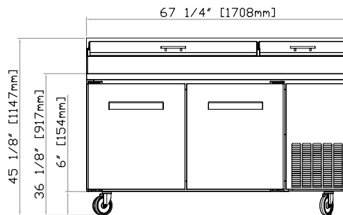
FPT-67 FRONT
